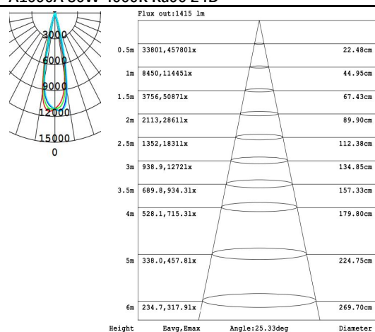
A1090A 30W 4000K Ra90 24D
