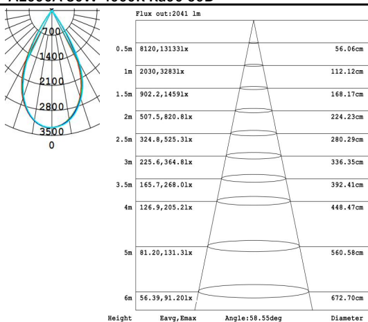
A1090A 30W 4000K Ra90 60D
