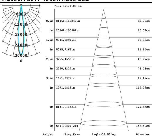
A1090A 30W 4000K Ra90 15D
