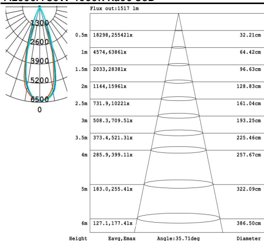
A1090A 30W 4000K Ra90 36D
